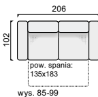
sofa SOF.2,5S
